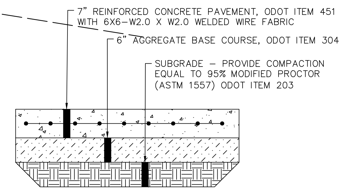
TYPICAL DRIVE SECTION DETAIL NO SCALE
